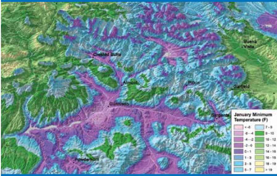
Figure 3. January 1971-2000 Minimum Temperature in the Gunnison, Colorado area.
