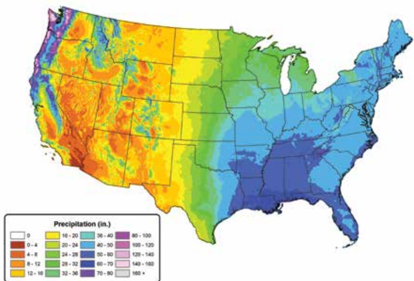
Figure 1. Precipitation: Annual Climatology (1981-2010)
