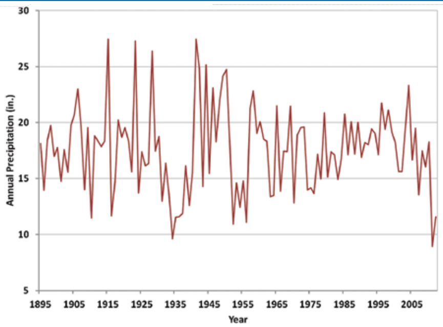
Figure 4. Annual Precipitation, 1895-2012: Texas County, Okla.
