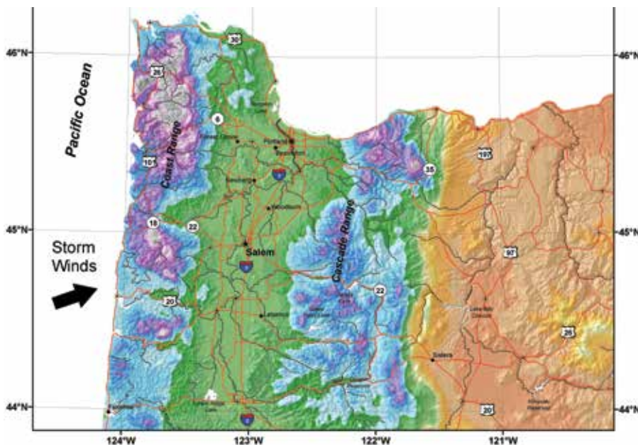
Figure 2. Oregon Annual Precipitation
